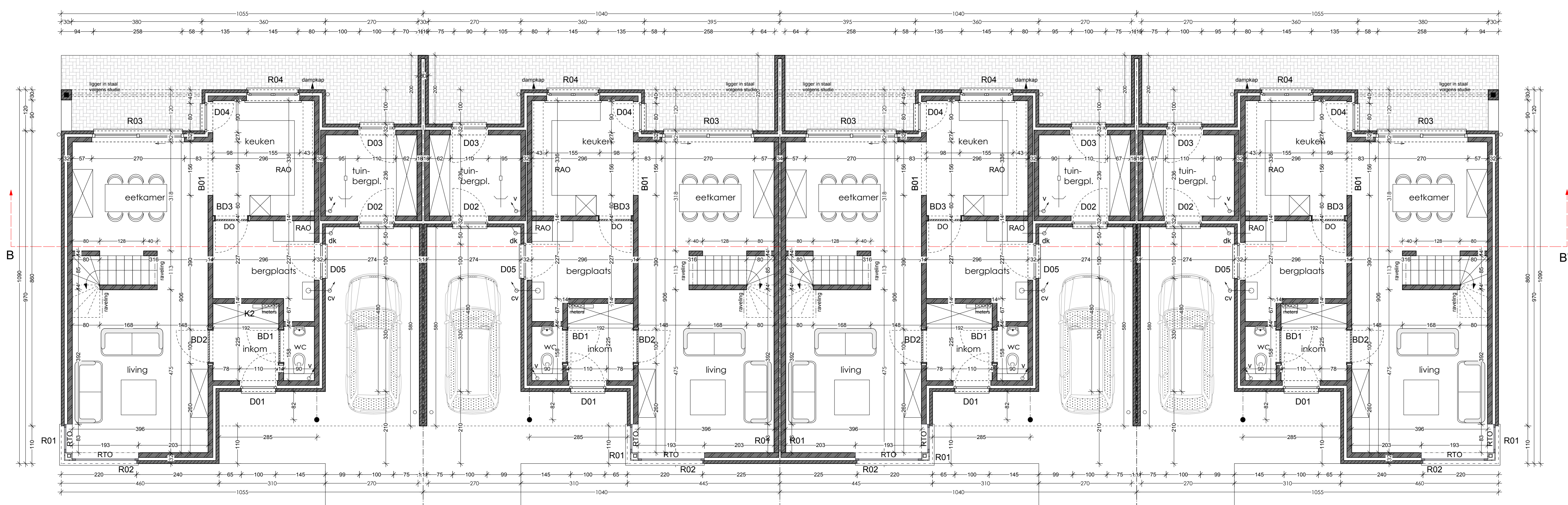
grondplan type 5 tem 8
